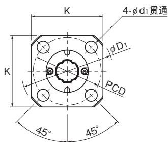
LFK5X~LFK8X
