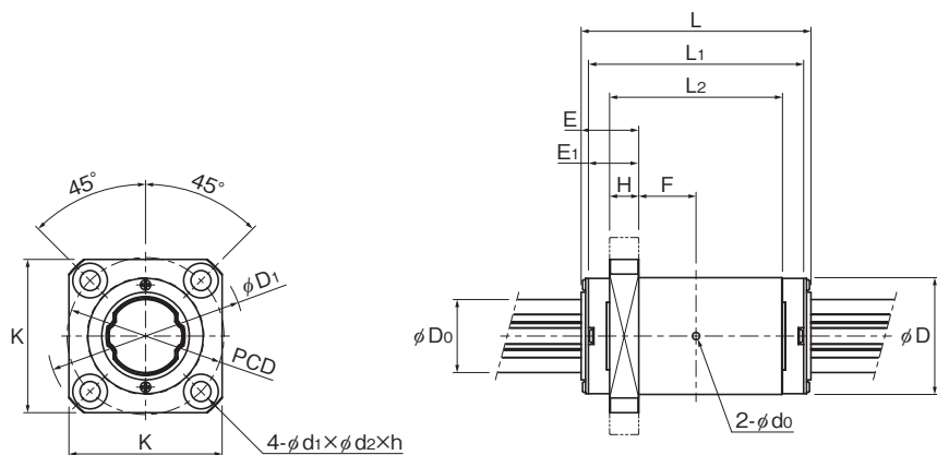
LFK10X~LFK30X
